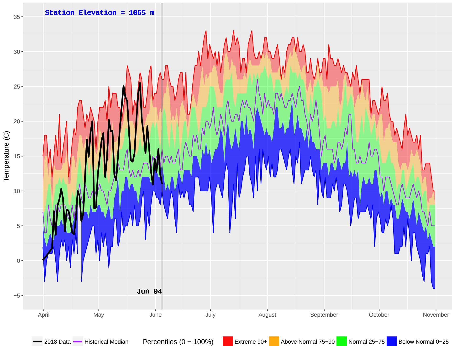
ASPEN GROVE (302) : Historical (1998–2016) and Current (2018) Noon Temperature
