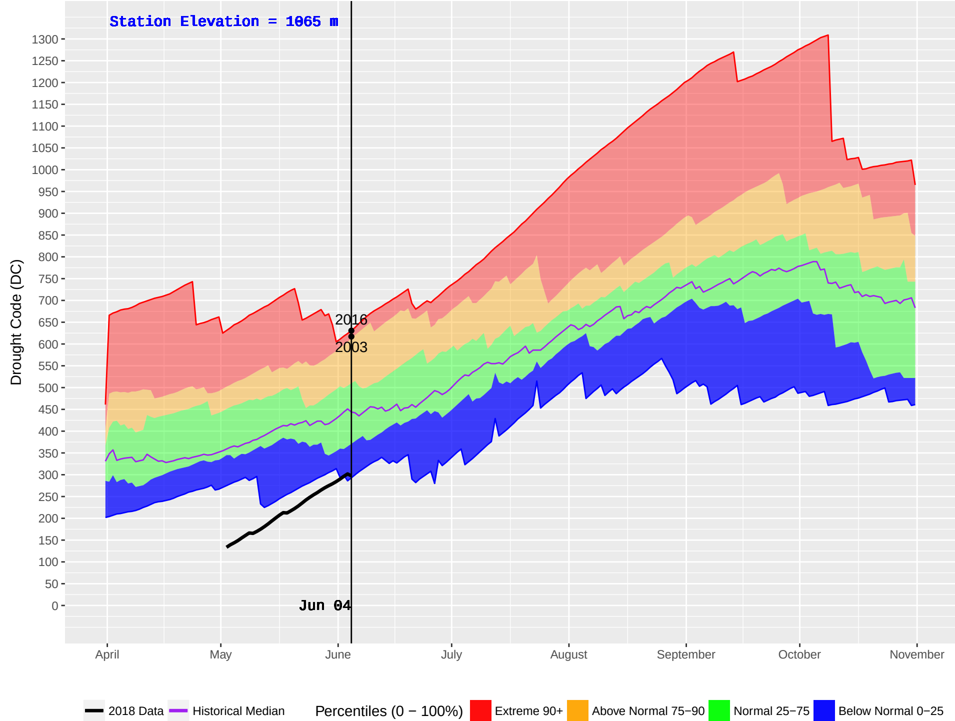
ASPEN GROVE (302) : Historical (1998–2016) and Current (2018) Noon Drought Code (DC)
